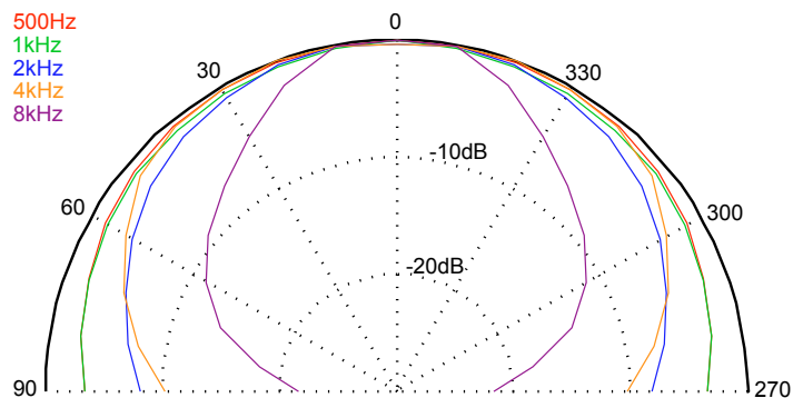
Figure 12 : Horizontal directivity (column SA250P/SA300P+)
