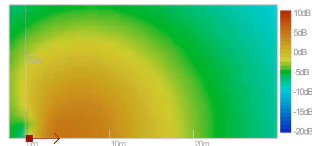
Figure 14 : SA100P / SA150P+ horizontal directivity: sound level for the voice octaves (500Hz,1kHz,2kHz) on the listening plane
