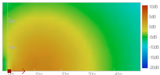
Figure 17 : SA180P / SA230P+ horizontal directivity: sound level for the voice octaves (500Hz,1kHz,2kHz) on the listening plane
