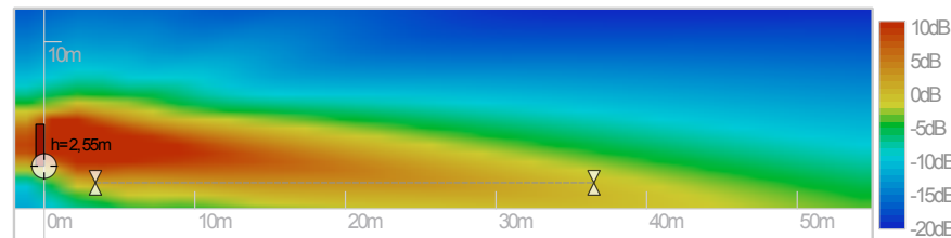
Figure 19 : SA250P / SA300P+ vertical directivity: sound level for the voice octaves (500Hz,1kHz,2kHz) in the vertical median plane
