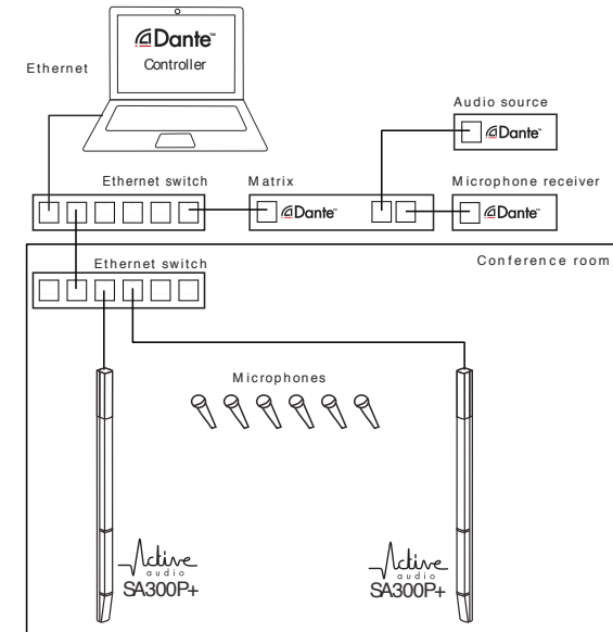
Figure 4 : StepArray+ setup using Dante network
