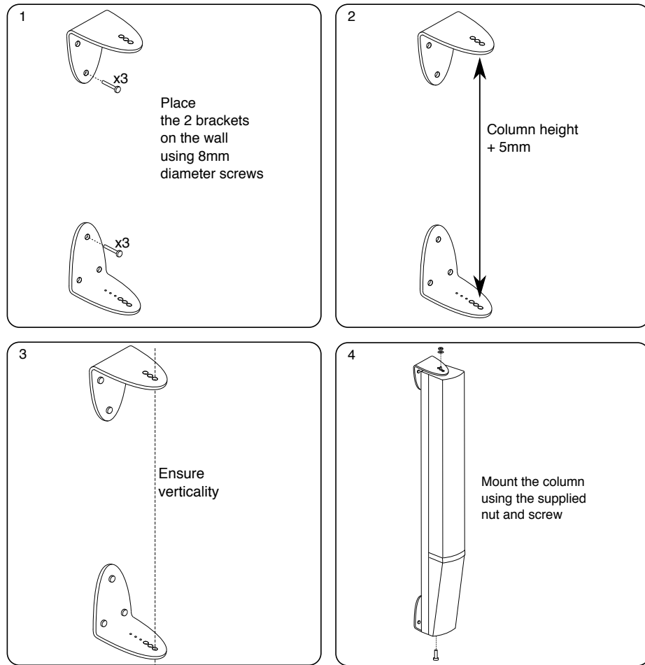
Figure 9 : Column mounting on a wall
