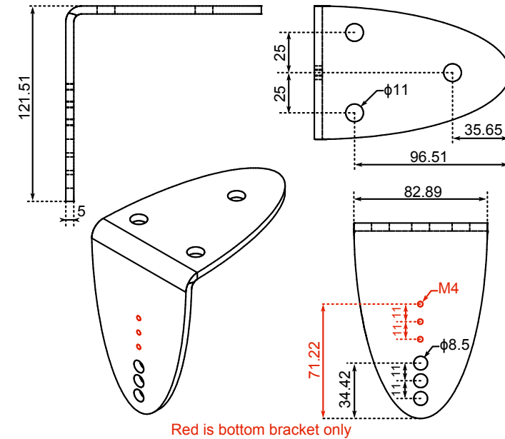
Figure 10 : Fixing brackets for wall mounting of StepArray columns
