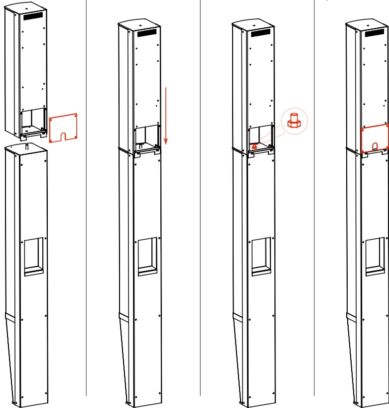
Figure 2 : Assembling StepArray+ columns
