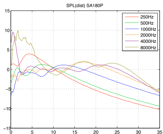
Figure 18 : Sound level by octave in the axis of the listening plane in front of the column with respect to the distance from the column
