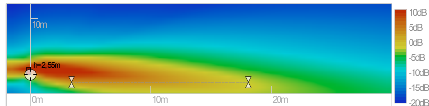
Figure 13 : SA100P / SA150P+ vertical directivity: sound level for the voice octaves (500Hz,1kHz,2kHz) in the vertical median plane
