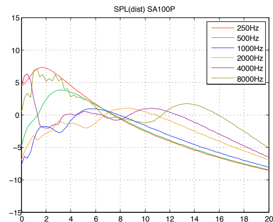
Figure 15 : Sound level by octave in the axis of the listening plane in front of the column with respect to the distance from the column
