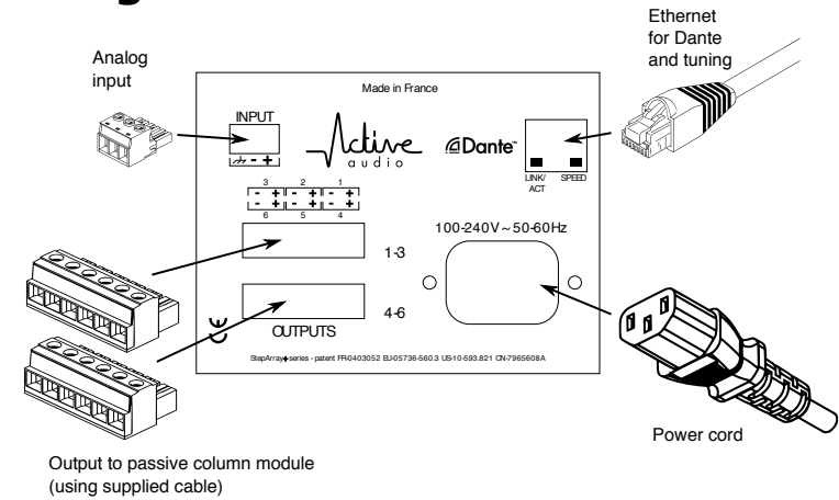
Figure 3 : Wiring StepArray+ columns
