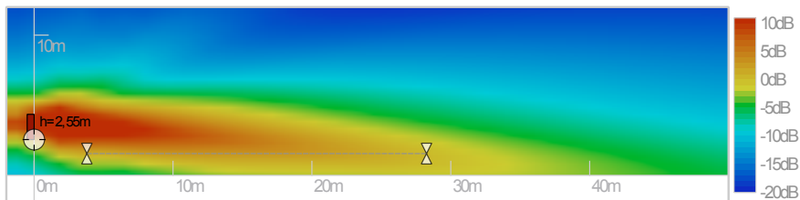
Figure 16 : SA180P / SA230P+ vertical directivity: sound level for the voice octaves (500Hz,1kHz,2kHz) in the vertical median plane
