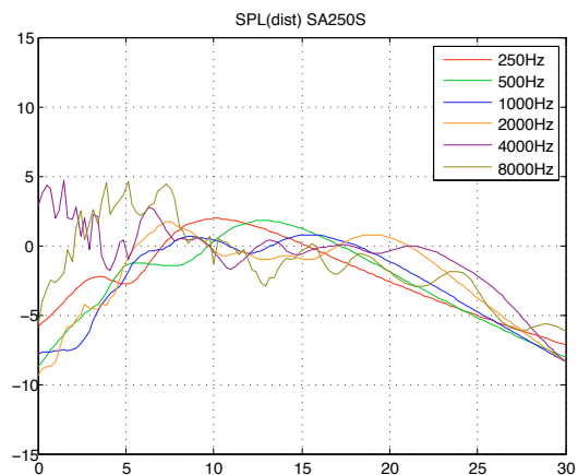
Figure 30 : Sound level by octave in the axis of the listening plane in front of the column with respect to the distance from the column
