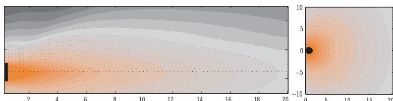
Standard 1m column vertical and horizontal directivity: sound level for the speech octaves (500Hz to 2kHz) in the vertical median plane.
