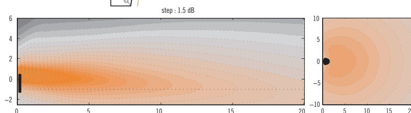
Ray-On R110 vertical and horizontal directivity: sound level for the speech octaves (500Hz to 2kHz) in the vertical median plane and 80cm below the column.
