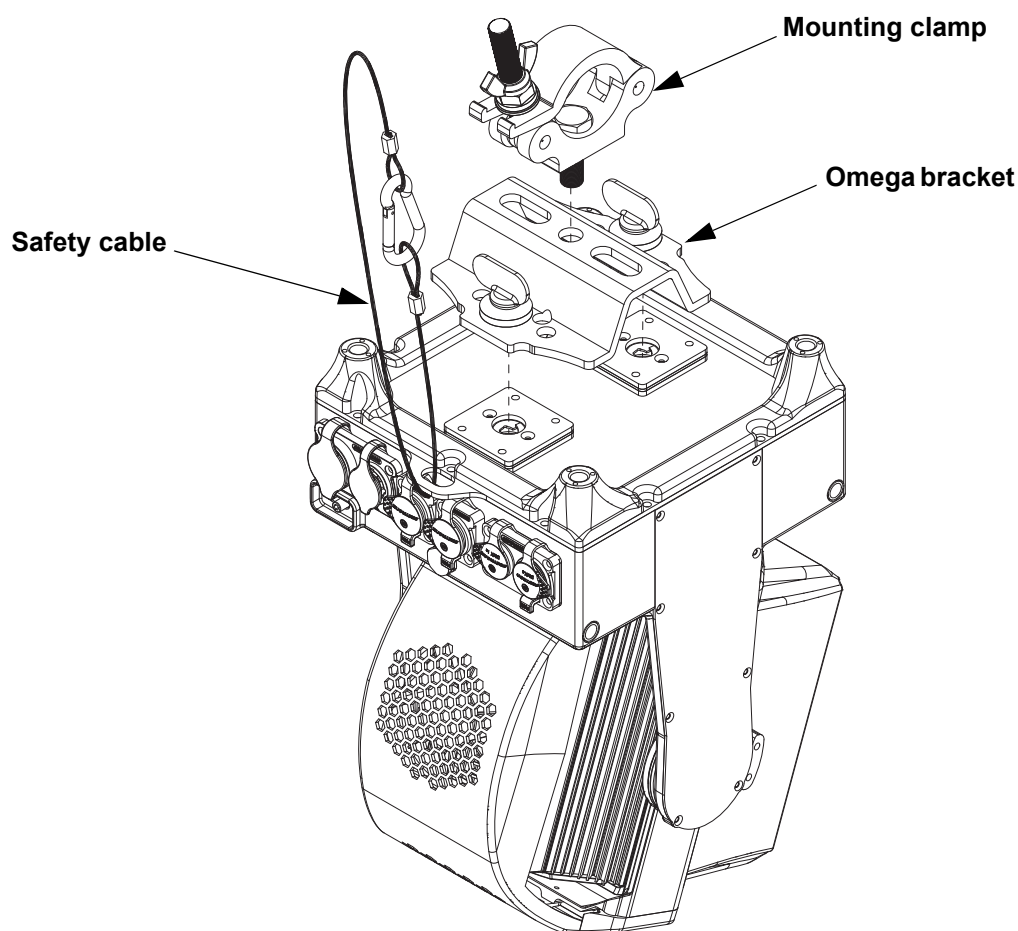
Overhead mounting
